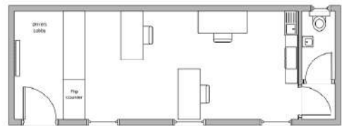
Transport Office Sample Layout 2 9m x 3m Transport Office With Drivers' Lobby, Open Plan Office, WC & Coffee Dock
