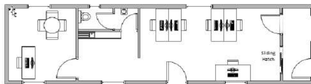
Transport Office Sample Layout 3 14.4m x 3.6m Transport Office With Drivers' Lobby, Open Plan Office, Private Offices, Meeting Room, WC & Coffee Dock
